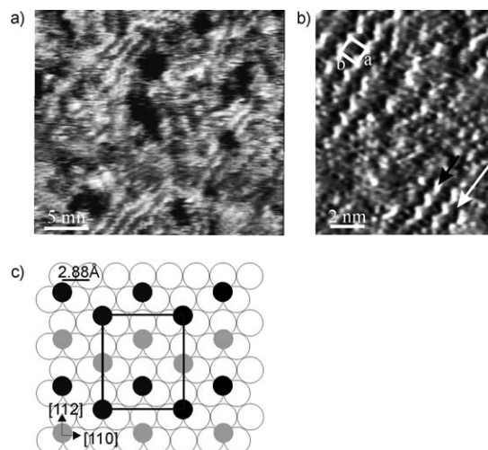
Figure 4. SAM formed after five days of incubation in a solution containing a 1/9 molar ratio of 1/2 . a) STM height contrast image; b) STM current contrast image; unit-cell parameters: a = (1.1 \pm 0.1) nm; b = (1.0 \pm 0.1) nm; \alpha = 92^\circ , area: 1.1 \text{ nm}^2 ( I_t = 2.172 \text{ pA} , V = 810 \text{ mV} ). c) Sketch of the molecular packing in the bicomponent domain.
